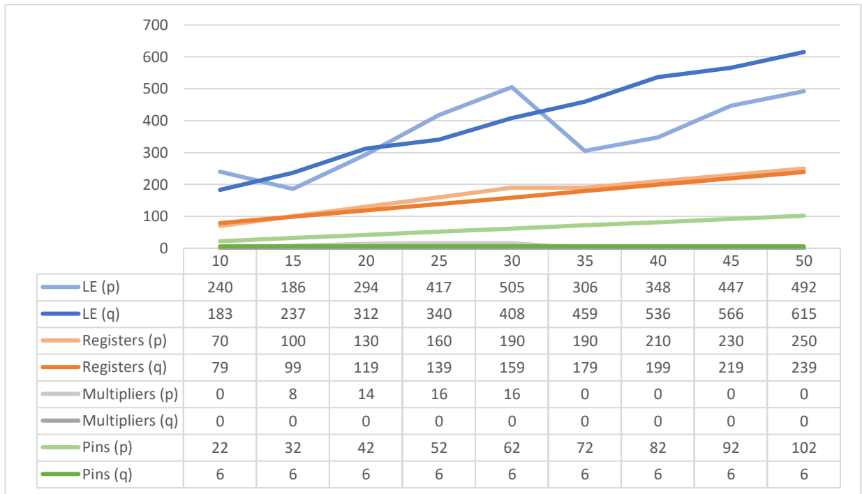
Fig. 4. Comparing the parallel (p) and quasiparallel (q) system in terms of resources used
