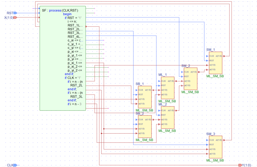
Fig. 2. Structure of the modular system
