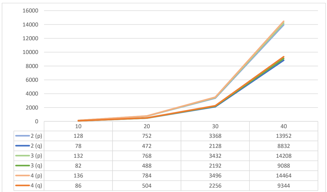
Fig. 5. Comparing the parallel (p) and quasiparallel (q) system in terms of number of iterations with on-line delay (p = 2, 3, 4)
